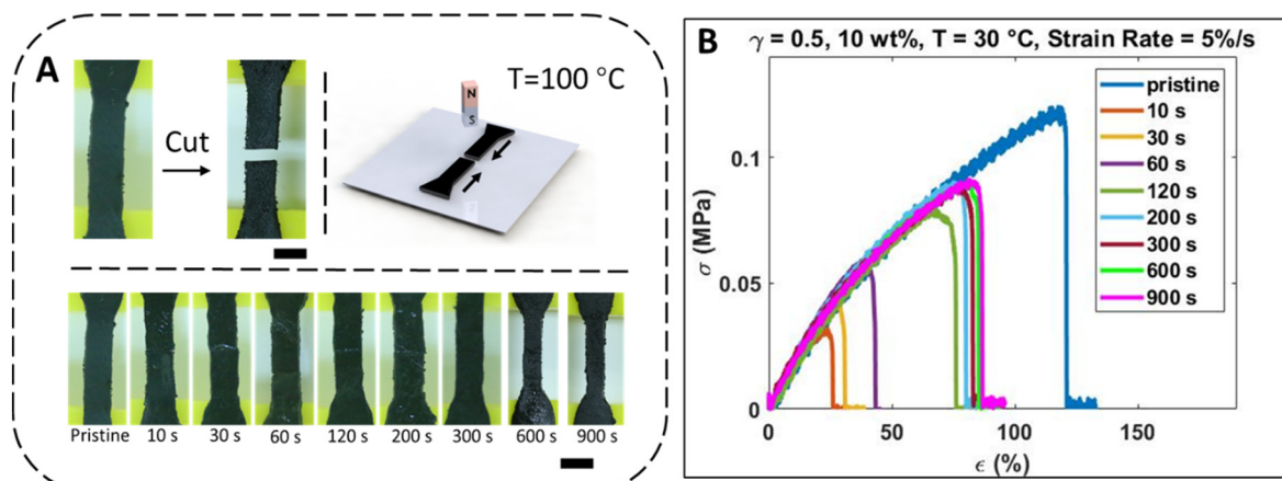
Fig. 5 Magnetically assisted self-healing of MV. (A) MV strips were first cut into two parts at 30\text{ }^{\circ}\text{C} . Then, assisted by the external magnetic field, the two broken parts were brought into contact and heated up at a temperature of 100\text{ }^{\circ}\text{C} to trigger the dynamic bond exchange reaction. Specimens were healed for different time periods. Scale bar, 2 mm. (B) Tensile stress–strain relationship of self-healed MV strips with different healing times.
