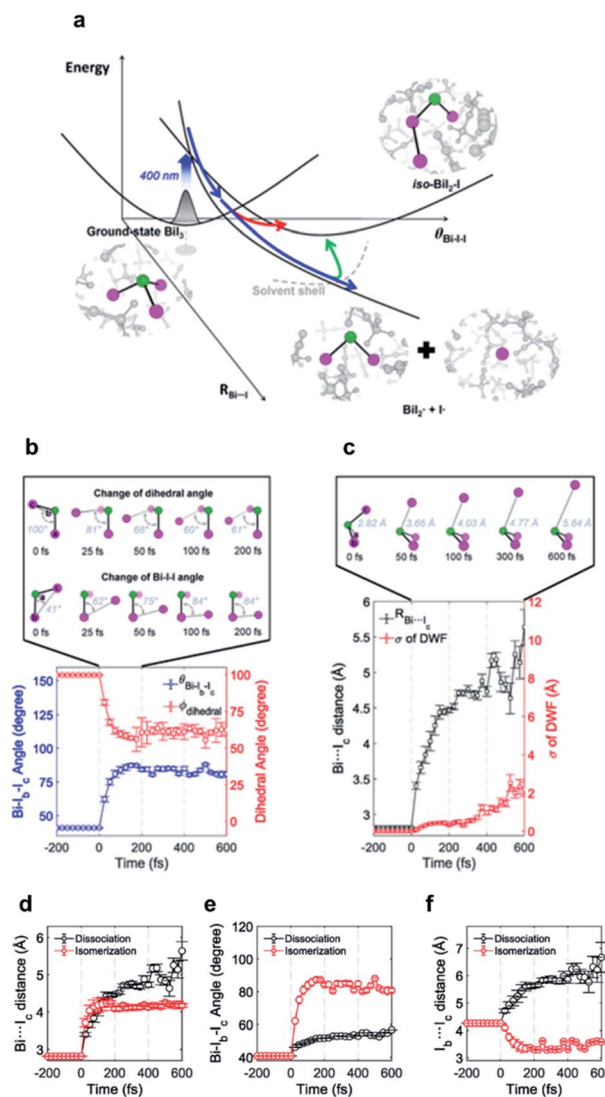
Fig. 3 (a) Schematic representation of the photodynamics of \text{BiI}_3 in acetonitrile. (b) Changes of the \text{Bi-I}_b-\text{I}_c angle and \text{I}_a-\text{Bi}-\text{I}_b-\text{I}_c dihedral angle during the roaming-mediated isomerization determined from structural analysis on the fs-TRXL data for \text{BiI}_3 in acetonitrile. (c) Changes of the \text{Bi}\cdots\text{I}_c distance and the root-mean-squared displacement ( \sigma ) associated with the pair distances containing \text{I}_c . Insets in (b) and (c) show transient structures at representative time delays. (d-f) Comparison of the structural motions for the dissociation and roaming-mediated isomerization channels through (d) \text{Bi}\cdots\text{I}_c distance, (e) \text{Bi-I}_b-\text{I}_c angle, and (f) \text{I}_b\cdots\text{I}_c distance. Reproduced from ref. 65 with the permission of Springer Nature, copyright 2021.
