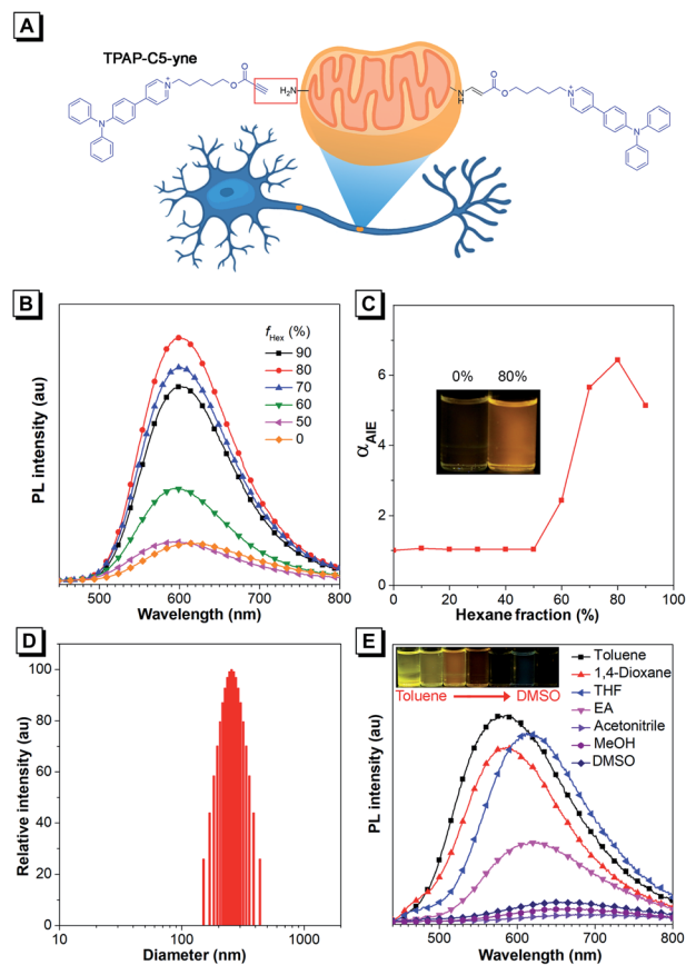
Fig. 1 (A) Structure of TPAP-C5-yne (left) and its bioconjugate after reacting with an amine group (right). (B) PL spectra of TPAP-C5-yne (10 μM) in THF and THF/hexane mixtures with different hexane fractions ( f_{\text{Hex}} ). (C) The plot of PL emission intensity versus the composition of the THF/hexane mixture containing TPAP-C5-yne. Inset: fluorescent photographs of TPAP-C5-yne in 0% and 80% hexane fractions under 365 nm UV irradiation. (D) Dynamic light scattering data of TPAP-C5-yne in THF/hexane mixtures containing 80% of hexane. (E) PL spectra of TPAP-C5-yne (10 μM) in different solvents.
