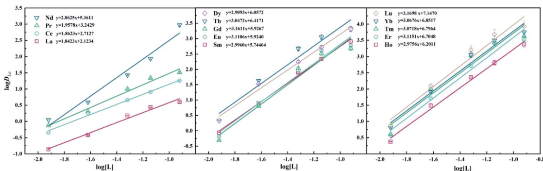
Fig. 4 Dependency of \log D_{\text{Ln}} on extractant concentration in 40/60 (v/v) n -octanol/kerosene (O : A = 1 : 1), [\text{Ln}^{3+}]_{\text{init}} = 3 \text{ mM} , [\text{L}^{II}] = 0.012 – 0.12 \text{ M} .
