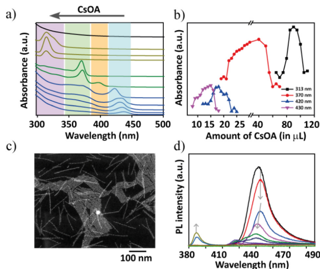
Fig. 2 (a) Absorption spectra of the transformation of Cs–(Pb)–Br nanostructures from \text{CsPbBr}_3 to \text{Cs}_4\text{PbBr}_6 NCs to \text{CsBr} NCs via the intermediate transient phase. The systematic trend of characteristic peak positions is labelled with different colours to represent the four major bands at \approx 430 nm, 420 nm, 370 nm, and 313 nm. The upper black trace is featureless, corresponding to \text{CsBr} NCs. The top arrow indicates the incremental addition of \text{P}_{\text{Cs-ol}} to the reaction. Titrations were carried out at RT and a constant concentration of the host, \text{P}_{\text{Pb-br}} . (b) The appearance of characteristic absorption bands ( \approx 430 nm, purple; 400 nm, blue; 370 nm, red; 313 nm, black) and their gradual progress during the titration of \text{P}_{\text{Cs-ol}} from 2 \mu\text{L} to 200 \mu\text{L} . (c) STEM image of the intermediate product formed between \text{CsPbBr}_3 and \text{Cs}_4\text{PbBr}_6 phases corresponding to the absorption at 370 nm, which persisted for a long titration period from 20 to 50 \mu\text{L} of \text{P}_{\text{Cs-ol}} addition (red trace in b). (d) The changes in PL intensity and the PL wavelength with respect to the titrations of (b).
