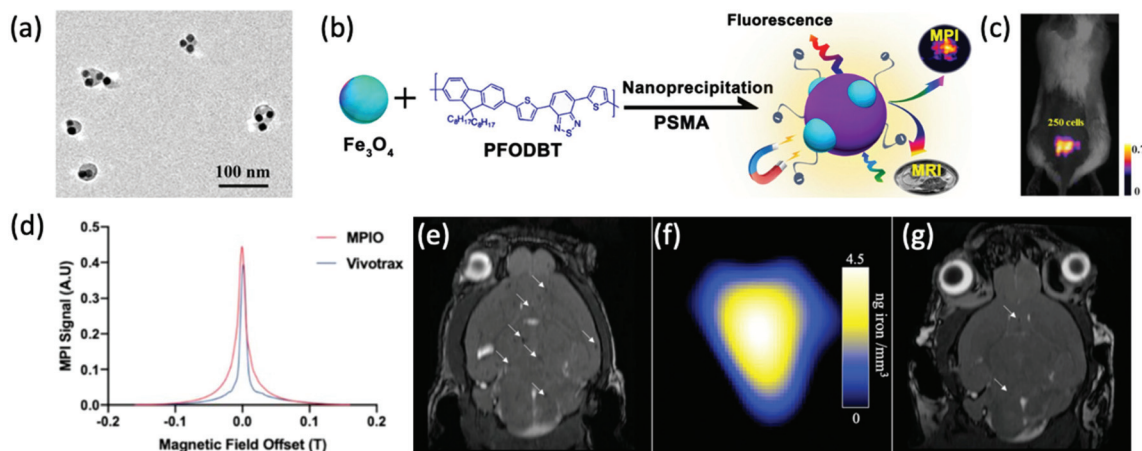
Fig. 13 The application of SPIONs in cancerous cell tracking with MPI. (a) TEM image of \text{Fe}_3\text{O}_4 @PFODBT–COOH Janus nanoparticles, where PFODBT is poly[2,7-(9,9-dioctylfluorene)- alt -4,7-bis(thiophen-2-yl)benzo-2,1,3-thiadiazole]. (b) Schematic demonstrating the synthetic preparation route of \text{Fe}_3\text{O}_4 @PFODBT–COOH Janus nanoparticles. (c) Overlay of a 2D projection MPI and white light image of a mouse implanted with 250 nanoparticle-labelled cells, following background subtraction. Reproduced with permission from ref. 12. Copyright 2018 American Chemical Society. (d) PSF demonstrating the MPI signal obtained for MPIO, in comparison to that of the reference, VivoTrax. The (e) MRI, and (f) MPI of a mouse brain injected with 5 \times 10^4 4T1BR5 cells labelled with VivoTrax. The (g) MRI, of a mouse brain injected with 5 \times 10^4 4T1BR5 cells labelled with MPIO. There was no MPI signal detected in the mouse brains injected with 5 \times 10^4 4T1BR5 cells labelled with VivoTrax. Reproduced with permission from ref. 29. Copyright 2020 the authors.
