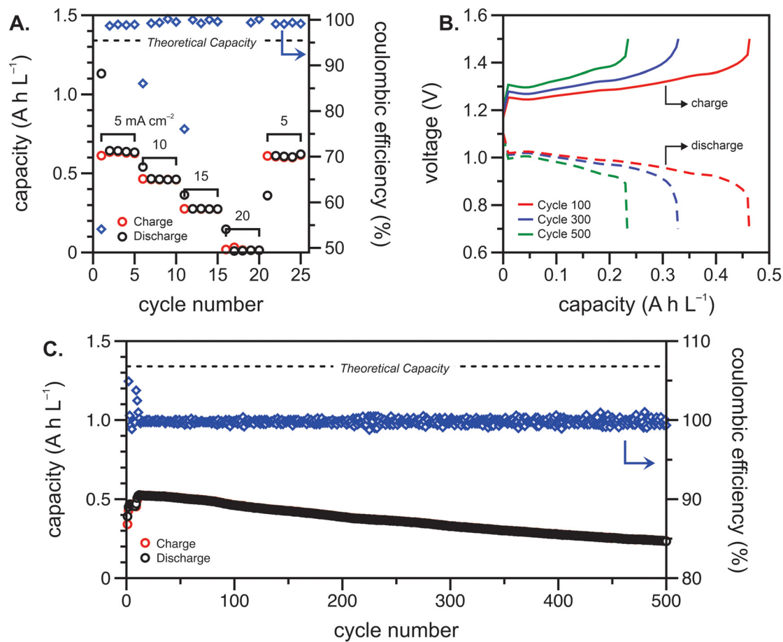
Fig. 4 Cycling of the polypeptide flow cell in a potential window of 0.7 to 1.5 V. (A) Capacity and coulombic efficiency vs. cycle number for current densities of 5, 10, 15, 20 and 5 \text{mA cm}^{-2} . (B) Galvanostatic charge/discharge curves taken at 100, 300, and 500 cycles. (C) Long-term cycling of the polypeptide flow cell. The current density for (B) and (C) was 10 \text{mA cm}^{-2} . The cell consisted of 7.5 mL each of 50 mM (by repeat unit) viologen polypeptide anolyte and 25 mM (by repeat unit) biTEMPO polypeptide catholyte in 0.5 M TEATFSI in ACN.
