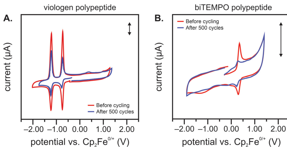
Fig. 5 Cyclic voltammetry at 100 \text{mV s}^{-1} of the (A) viologen polypeptide anolyte and (B) biTEMPO polypeptide catholyte before and after cycling of the polypeptide redox flow cell (arrows denote 10 \mu\text{A} ). Glassy carbon was used as the working electrode, platinum wire as the counter electrode, un-fritted freshly anodized Ag/AgCl wire as the reference electrode, and ferrocene was used as internal reference. The supporting electrolyte was 0.5 M TEATFSI in ACN.
