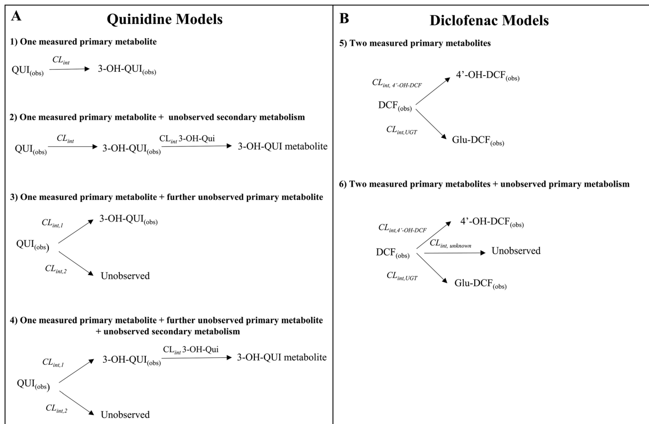
Fig. 7 A) Schematic representation of the metabolic pathways investigated with the in silico model for the experimental data of quinidine. B) In silico models for the f_{\text{m,UGT}} and estimation of diclofenac. The subscript Obs refers to the measured medium concentration of the respective compound.
