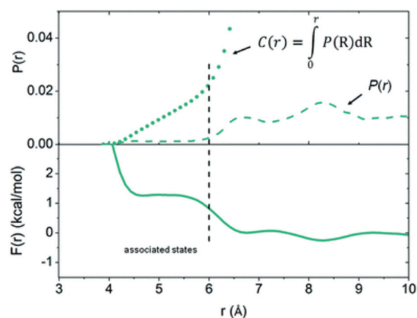
Fig. 2 Free energy curve, F(r) , and probability distribution, P(r) , computed from MD simulations of \text{P}(\text{tBu})_3/\text{B}(\text{C}_6\text{F}_5)_3 in toluene. Reproduced from ref. 67 with permission from the Royal Society of Chemistry.
