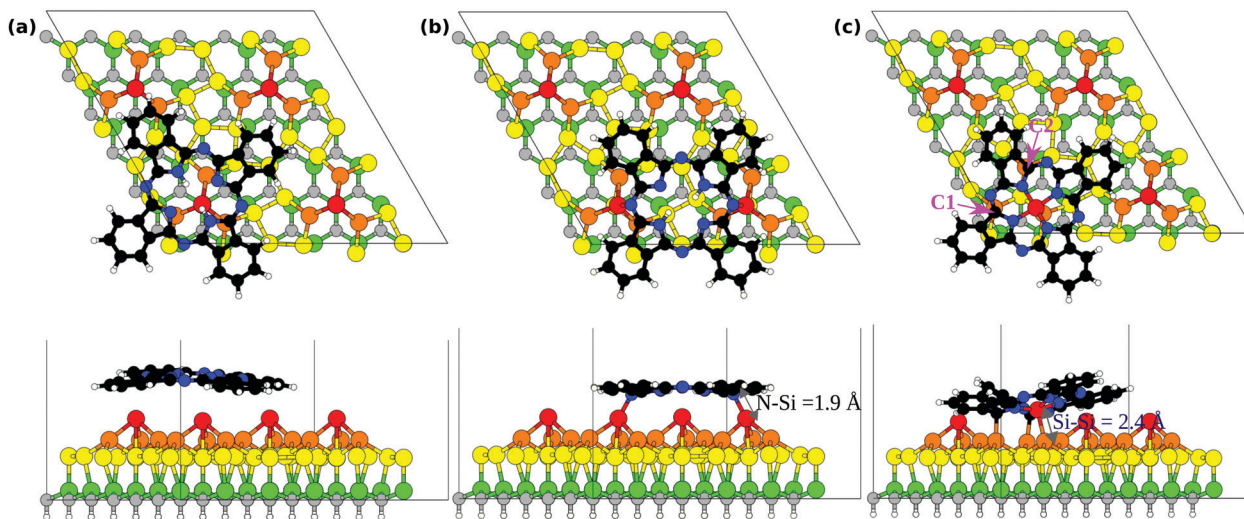
Fig. 7 Optimized configurations obtained for (a) top and (b) bridge positions of \text{H}_2\text{Pc}/6\text{H-SiC}(0001)-(3 \times 3) , (c) top positioned \text{SiPc}/6\text{H-SiC}(0001)-(3 \times 3) . The top panel shows the top view and the bottom panel shows the side view. The molecule is colored as follows: C-black, N-blue, H-white, and Si-red. The substrate is colored as follows: Si adatoms (first layer S1)-red, Si trimers (second layer S2)-orange, Si (third layer S3)-yellow, Si (fourth layer)-green, C-grey, and H-white.
