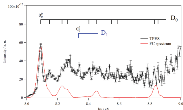
Fig. 3 TPES spectrum of 9\text{MA} in the 8–9 eV region. Also shown is a Franck–Condon simulated spectrum set to an absolute scale via high level computations’-determined AIE. The vertical combs correspond to the peak positions reported in Table 4.
