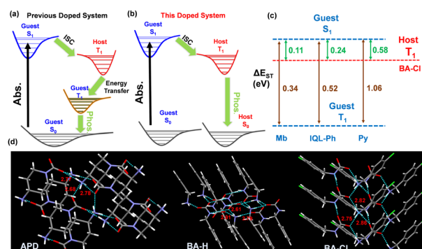
Fig. 3 (a) Proposed luminescence mechanism of the previous doped system. (b) Proposed luminescence mechanism of this doped system. (c) \Delta E_{ST} of the guest and the hosts. (d) Single crystal structures of APD , BA-H , and BA-Cl (the cyan dotted lines represent hydrogen bonds, and the red numbers represent the distance of hydrogen bonds. CCDC: 2189315 of APD , 2189318 of BA-H , 2189320 of BA-Cl ). †
