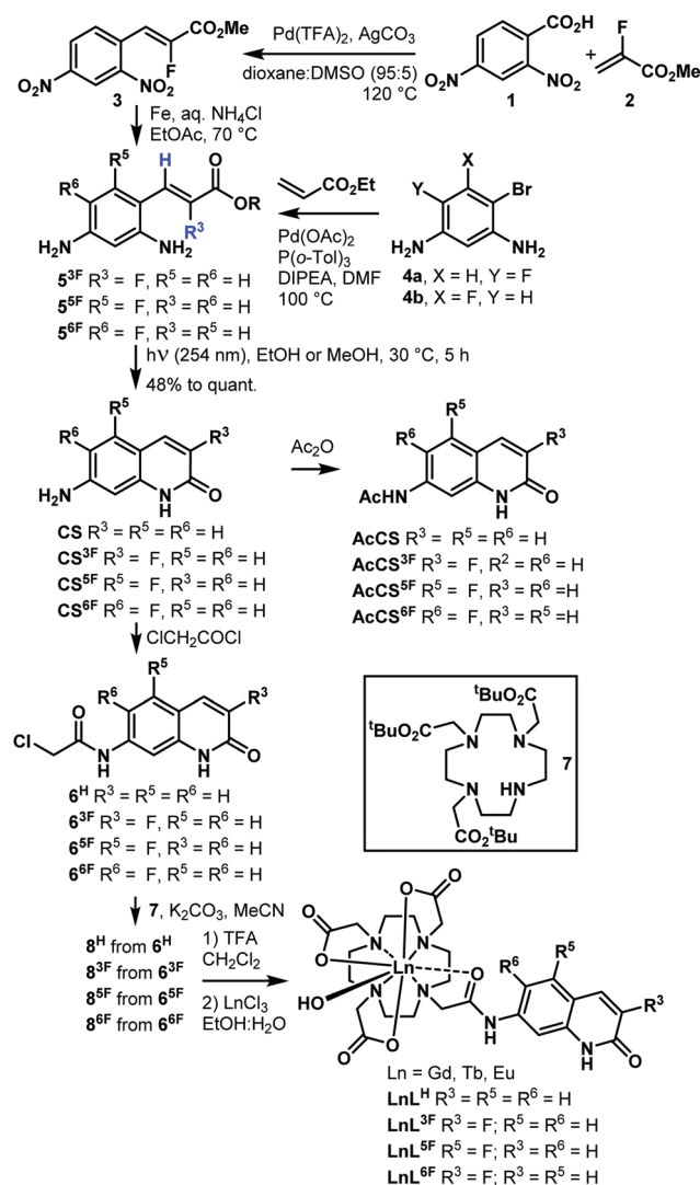
Scheme 1 Preparation of \text{CS}^{\text{F}} , \text{AcCS}^{\text{F}} , \text{AcCS}^{\text{F}} , and \text{LnL}^{\text{F}} .
