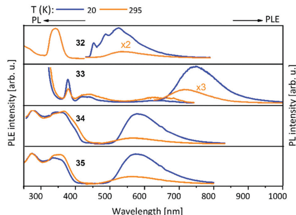
Fig. 10 Solid state excitation and emission spectra of PN 4 ( L 12 ) metal complexes 32–35 . PL was excited at \lambda_{\text{exc}} = 350 nm and PLE spectra recorded at \lambda_{\text{em}} = 560 nm for 32 , 33 , 35 and \lambda_{\text{em}} = 580 nm for 34 . 48
