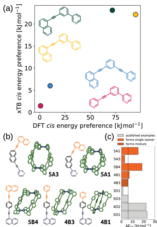
Fig. 9 (a) Comparison of GFN2-xTB (DMSO) and DFT (PBE0/def2-SVP/D3BJ/CPCM(DMSO)) energy difference between the cis stable isomer of cages formed in ref. 121 from the ligands 3D1 (crimson), 4D2 (yellow), 5D1 (dark green) and 5D3 (blue). (b) GFN2-xTB optimised structure of the cis isomer of selected cage ligands (hydrogen atoms omitted; C green, N blue, Pd cyan). Cage ligands are shown next to each structure with orange and navy indicating inequivalent ligand fragments. (c) cis isomer GFN2-xTB (DMSO) stability (ΔE cis ) for all published 121 and newly selected ligands (patterns distinguish their self-assembly outcomes). Adapted from ref. 99.
