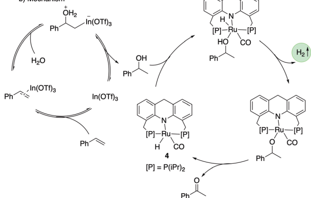
Fig. 21 (a) Alkene oxidation to a ketone with water catalyzed by 4. (b) Reaction mechanism.
