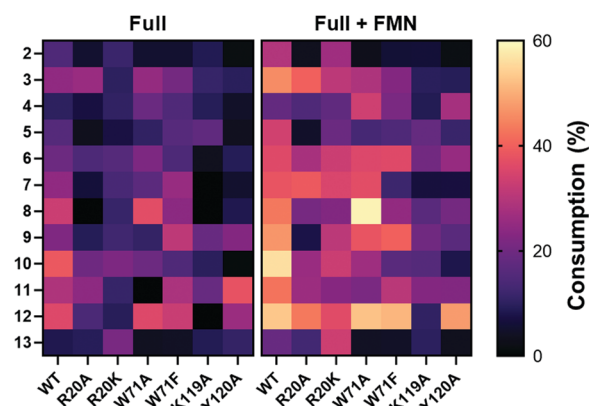
Fig. 7 Heat map of the consumption of compounds 2–13 by WT HiNfsB and its R20A, R20K, W71A, W71F, K119A and Y120A mutants. The reactions contained 2 mM substrate, 0.1 \mu M enzyme, 1 mM NADP + , 20 mM glucose, and 16 \mu M GDH in 100 mM phosphate buffer (pH 7.4) and were incubated at room temperature for 10 min. The data represent means \pm s.d. of three independent experiments.
