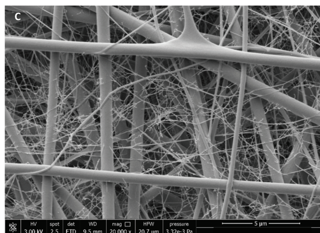
Fig. 3 (A) Fiber diameter of PCL specimens with 7.5/10/12.5%, 10/15/20/25 kV and 20 cm spinning distance; (B) fiber diameter of SF-PCL specimens with 0/33/50/66% SF, 10% polymer concentration, 20 kV and 15 cm spinning distance (large fiber fraction); (C) SEM image of SF-PCL 1:2, 10%, 20 kV, 15 cm with bimodal fiber diameter distribution, scale bar 5 \mu\text{m} ; ** p < 0.01 .
