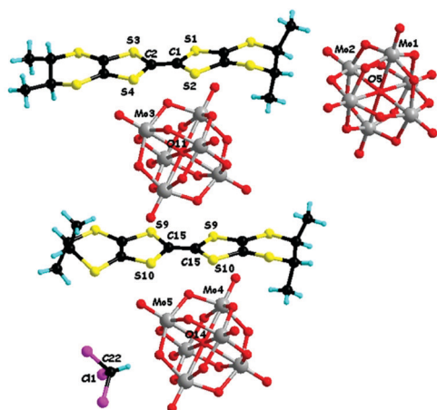
Fig. 1 Detail of the crystal structure of [(S)-1]_9(Mo_6O_{19})_5 \cdot (CHCl_3)_2 with the two different donors (one and half independent), three different polyoxometallate dianions (two one third and one sixth independent) and a CHCl_3 solvent molecule (one third independent).
