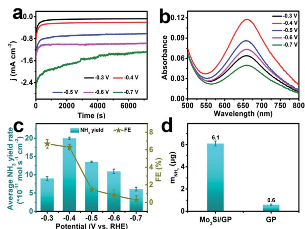
Fig. 2 (a) Time-dependent current density curves of \text{Mo}_3\text{Si}/\text{GP} at different potentials in 0.1 M \text{Na}_2\text{SO}_4 . (b) UV-Vis absorption spectra of the electrolytes stained with the indophenol indicator after electrolysis at a series of potentials for 2 h. (c) Corresponding average \text{NH}_3 yield rate and FEs of \text{Mo}_3\text{Si}/\text{GP} at all potentials. (d) Amount of \text{NH}_3 produced for \text{Mo}_3\text{Si}/\text{GP} and GP after charging at -0.4 \text{ V} for 2 h in 0.1 M \text{Na}_2\text{SO}_4 .
