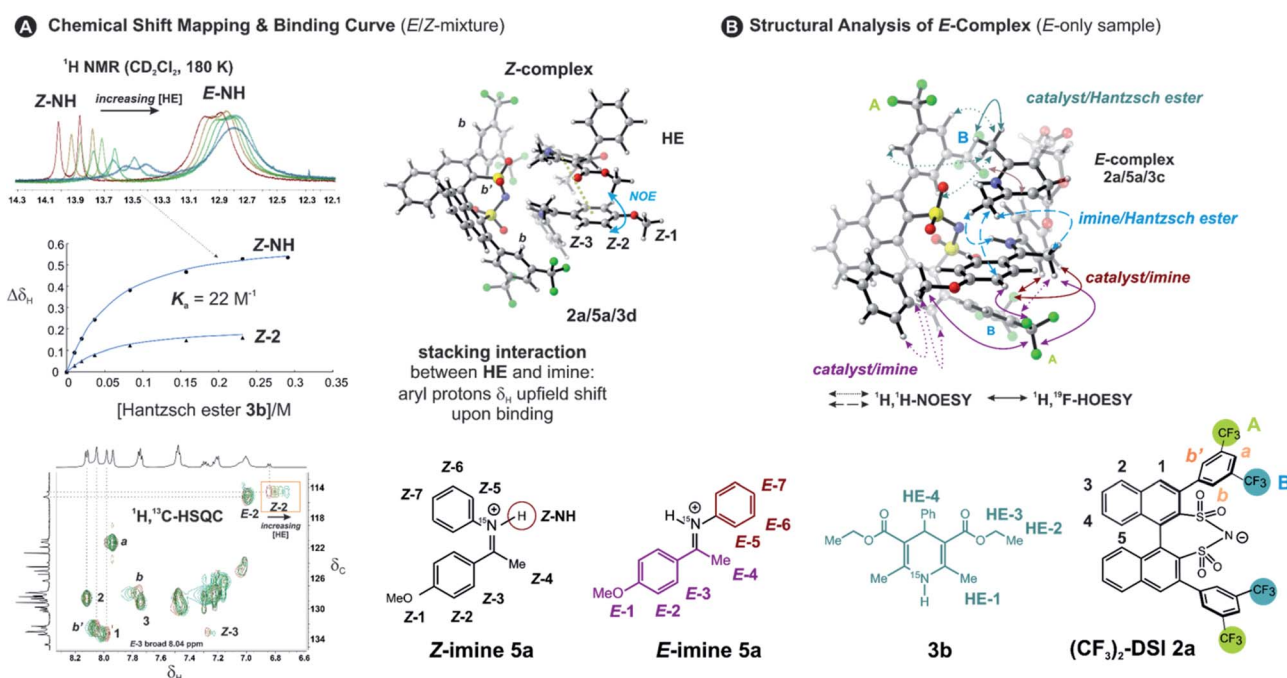
Fig. 2 Chemical shift mapping and NOE/HOE analysis proves bifunctional binding in the ternary complex: (A) stronger binding of Z -imine from chemical shift mapping; titration of (\text{CF}_3)_2 -DSI 2a/5a E/Z mixture (20 mM) with 0–15 eq. Hantzsch ester 3b , followed by ^1\text{H} NMR and ^1\text{H},^{13}\text{C} -HSQC spectra in \text{CD}_2\text{Cl}_2 at 180 K (NH signals split into doublets by ^1J_{\text{NH}} due to the iminium ^{15}\text{N} nucleus). Fitting of the \Delta\delta_{\text{H}} ( Z -NH and Z -2) gave a binding constant K_a = 22 \text{ M}^{-1} for Z - 5a . The plausible calculated structure 2a/5a/3d (TPSS-D3(BJ)/def2-SVP/SMD( \text{CH}_2\text{Cl}_2 )) shows the NOE contact and explains the most pronounced chemical shift differences for Z -2/ Z -3 resonances upon binding. (B) A plausible calculated structure of ternary of E -complex 2a/5a with Hantzsch ester 3c with key NOE and HOE contacts shown.
