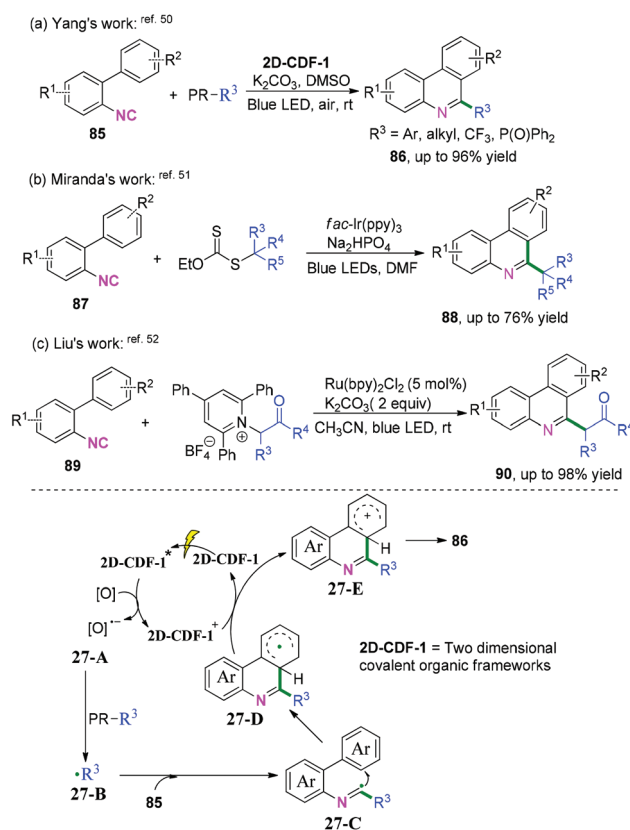
Scheme 41 Visible-light-induced cascade radical cyclization of 2-substituted phenyl isocyanides.
