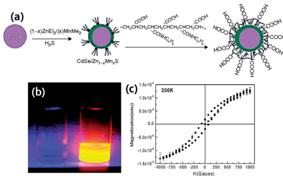
Fig. 2 (a) Synthesis procedure for the fabrication of water soluble core/shell CdSe/Zn 1-x Mn x S. Reproduced from ref. 65 with permission from American Chemical Society, copyright 2007. (b) Fluorescence of yellow-emitting QDs (right) and DI water (left) under 366 nm UV source and (c) magnetization curve for QDs. Reproduced from ref. 70 with permission from American Chemical Society, copyright 2005.
