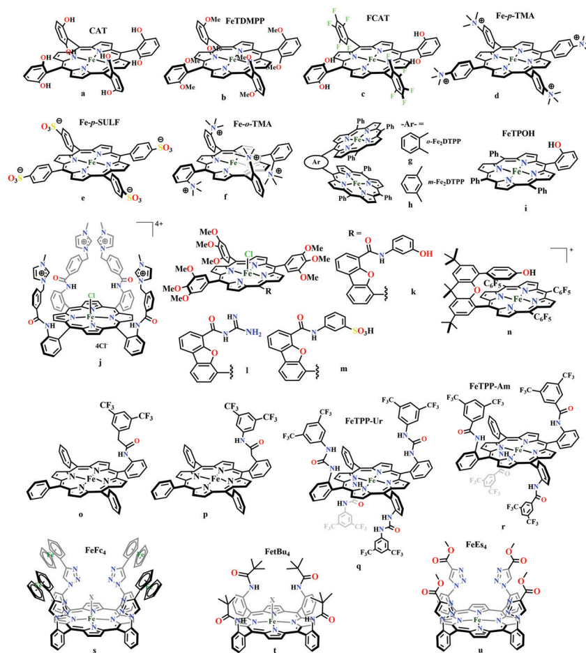
Fig. 7i). 116 The Fe-TPOH complex was shown to reduce CO 2 to CO (96% FE) at TOF ~ 4500 s -1 in acetonitrile in presence of weak Brønsted acids (1 M water or 8 mM phenol). In contrast, the catalyst was found to be very poor in DMF. Based of Abraham's H-bond acidity 117 and basicity 118 as metrics, it has been suggested that DMF being a strong H-bond acceptor, plays a detrimental role in catalysis, where H-bonding is very crucial in accelerating the rate. Substituting the four meso-p -hydrogens of FeTPP by trimethylammonium groups (WSCAT) could afford formation of a water-soluble porphyrin (Fig. 7d). Under neutral pH, it catalyzes the reduction of CO 2 to CO, selectively. 119
