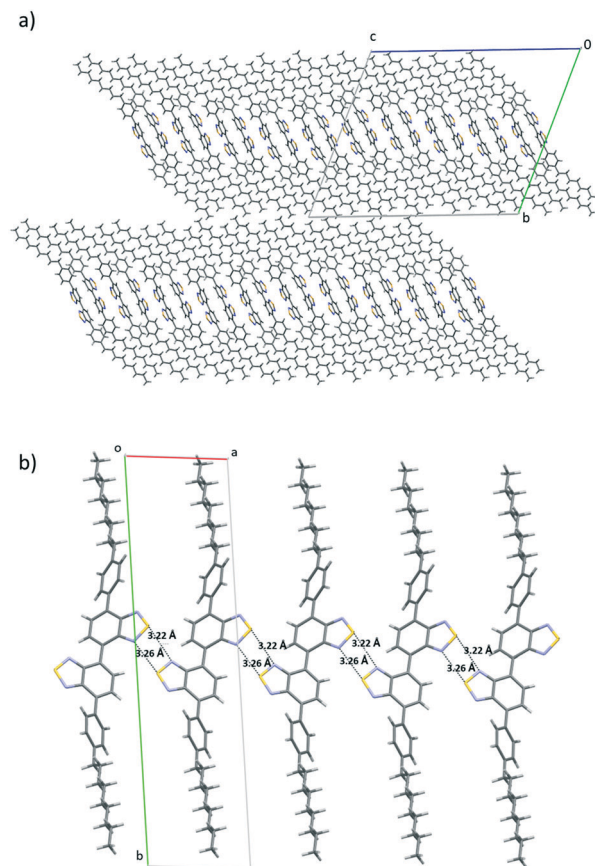
Fig. 2 a) A view of the crystallographic packing of 4 showing the layered arrangement. b) A view of the sheets that form the layer growing along the a direction interacting through chalcogen bonding 2\text{S}–2\text{N} squares.
