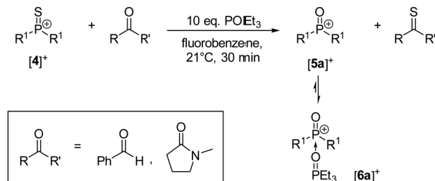
Scheme 3 Conversion of carbonyls to thiocarbonyls using [4][BARF 24 ] and POEt 3 as trapping reagent. [BARF 24 ] − anions are omitted for clarity.
