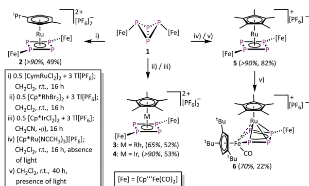
Scheme 2 Synthesis of the isomerisation products starting from 1 . The yields in italics are based on the ^{31}P NMR spectra of the crude reaction mixture, while the second value refers to the isolated yield.
