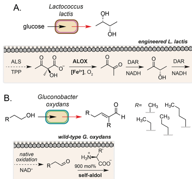
Fig. 4 Intracellular non-enzymatic catalysis for production of high value small molecules. (A) \text{Fe}(\text{II}) -catalysed non-enzymatic oxidative decarboxylation (ALOX) of acetolactate in L. lactis enables efficient access to diacetyl, acetoin and butanediol. DAR refers to diacetyl reductase from Enterobacter cloacae . (B) Native oxidation of short chain alcohols by G. oxydans coupled with an organocatalytic aldol condensation gives access to valuable \alpha,\beta -unsaturated compounds.
