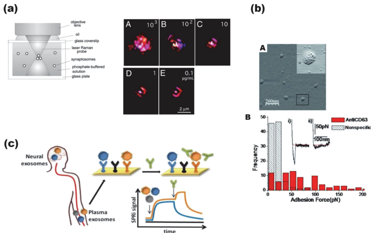
Fig. 6 (a) Optical set up for laser trapping of subcellular vesicles during laser-trapping. Imaging of reflected light from different quantities – (A) 10^3 , (B) 10^2 , (C) 10, (D) 1, and (E) 0.1 – of aggregated and single subcellular vesicles during laser-trapping. Adapted from ref. 133 with permission from Royal Society of Chemistry, Copyright 2002. (b) Atomic force microscopy (AFM) imaging of exosomes with CD63 surface expression. (A) Image of 5–8 nm antibody-functionalized gold beads bound specifically to exosomes, inset shows a single exosome with surface-bound gold beads. (B) Distribution of rupture events by interaction forces between (i) antiCD63-coated or (ii) non-specific antibody-functionalized AFM tips and the exosome surface. Adapted from ref. 141 with permission from American Chemical Society, Copyright 2010. (c) Surface plasmon resonance imaging that uses antibodies against CD81 and GM1 for characterization of multiple exosome subpopulations in blood. Adapted from ref. 151 with permission from American Chemical Society, Copyright 2018.
