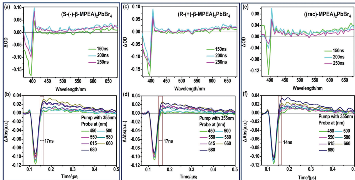
Fig. 3 ns-TA spectra of (a) (S-β-MPEA) 2 PbBr 4 , (c) (R-β-MPEA) 2 PbBr 4 , (e) ((rac)-MPEA) 2 PbBr 4 films upon excitation at 355 nm. TA onsets of (b) (S-β-MPEA) 2 PbBr 4 (d) (R-β-MPEA) 2 PbBr 4 , (f) ((rac)-MPEA) 2 PbBr 4 films probed at different wavelength.
