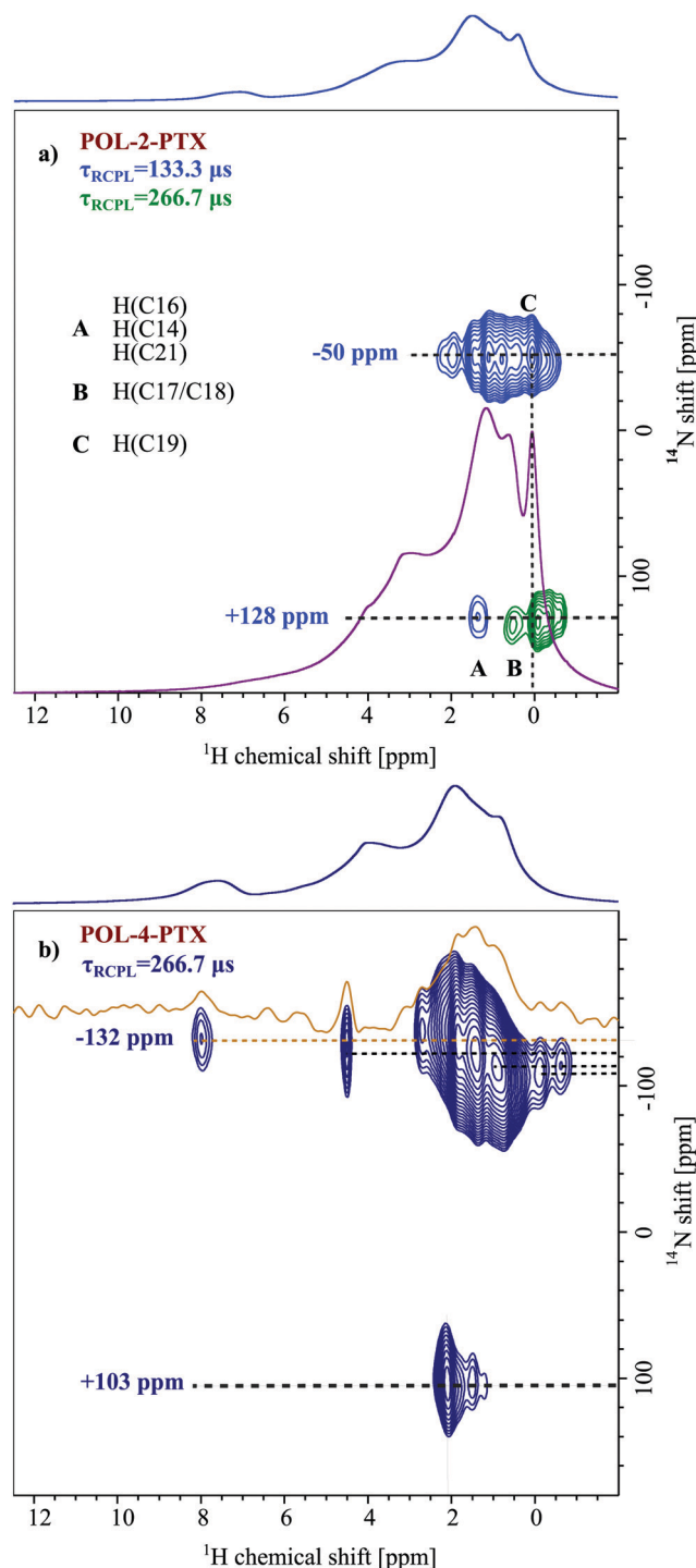
Fig. 3 ^{14}\text{N} - ^1\text{H} HMQC spectra (20 T, 60 kHz) of (a) the POL-2-PTX formulation recorded with recoupling times \tau_{\text{RCP1}} = 133.3 \mu\text{s} (light blue) and \tau_{\text{RCP1}} = 266.7 \mu\text{s} (green), both acquired with 18 t_1 FIDs, each with 1024 co-added transients for a recycle delay of 1.3 s (experimental time: 6 h 46 min), including tentative assignment of \text{N}\cdots\text{H} proximities. The base contour level is at 34% of the maximum peak height. The internal overlaid ^1\text{H} spectrum (purple) is that for POL. (b) The POL-4-PTX formulation recorded with a recoupling time \tau_{\text{RCP1}} = 266.7 \mu\text{s} (dark blue), and 12 t_1 FIDs each acquired with 1200 co-added transients for a recycle delay of 1.3 s (experimental time: 5 h 17 min). The internal overlaid spectrum (orange) is the extracted slice at a ^{14}\text{N} shift of -132 \text{ ppm} . The base contour level is at 22% of the maximum peak height. The skyline projections represent the ^1\text{H} one-pulse MAS NMR spectra of each sample.
