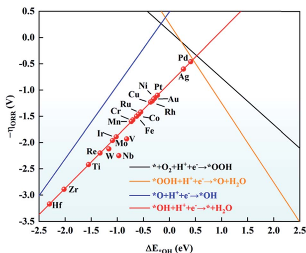
Fig. 6 Relationship between the negative of overpotential ( -\eta_{\text{ORR}} ) and the adsorption energy of OH ( \Delta E_{*OH} ). Each line denotes one reaction step acquired from the scaling relationships, * + \text{O}_2 + \text{H}^+ + \text{e}^- \rightarrow * \text{OOH} (in black): -\eta_{\text{ORR}} = -0.89\Delta E_{*OH} + 0.12 ; * \text{OOH} + \text{H}^+ + \text{e}^- \rightarrow * \text{O} + \text{H}_2\text{O} (in yellow): -\eta_{\text{ORR}} = -1.51\Delta E_{*OH} + 0.26 ; * \text{O} + \text{H}^+ + \text{e}^- \rightarrow * \text{OH} (in blue): -\eta_{\text{ORR}} = 1.40\Delta E_{*OH} + 0.49 ; * \text{OH} + \text{H}^+ + \text{e}^- \rightarrow * + \text{H}_2\text{O} (in red): -\eta_{\text{ORR}} = \Delta E_{*OH} - 0.87 .
