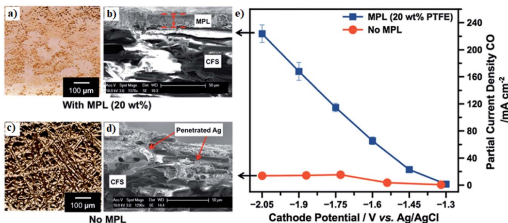
Fig. 10 (a and c) Micro-computed tomography and (b and d) SEM images of Ag-based GDE with and without the microporous layer. (e) A comparison of CO partial CD of Ag-based GDE with and without MPL as a function of potential. Reprinted with permission from Kim et al. , 162 Copyright 2016, Elsevier Ltd.
