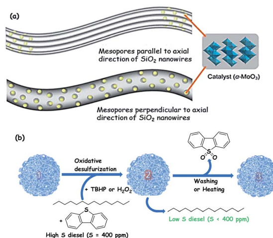
Fig. 8 (a) Illustrations of catalyst nanoparticles loaded via two different routes in the mesoporous \text{SiO}_2 nanowires (mesopores parallel to the axial direction of \text{SiO}_2 nanowires and mesopores perpendicular to the axial direction of \text{SiO}_2 nanowires). (b) Dual functions (catalyst + adsorbent) of \text{Mo}/m\text{SiO}_2 ( m denotes mesoporous) in the present investigation of the oxidative desulfurization process (1): fresh \text{Mo}/m\text{SiO}_2 nanowires, (2): dibenzothiophene sulfone adsorbed \text{Mo}/m\text{SiO}_2 nanowires, and (3): washed \text{Mo}/m\text{SiO}_2 nanowires ( i.e. , equivalent to 1); intricate thin threads represent networked \text{Mo}/m\text{SiO}_2 nanowires with mesopores perpendicular to the axial direction (which is detailed in (a)). Adapted from ref. 33 with permission from The American Chemical Society.
