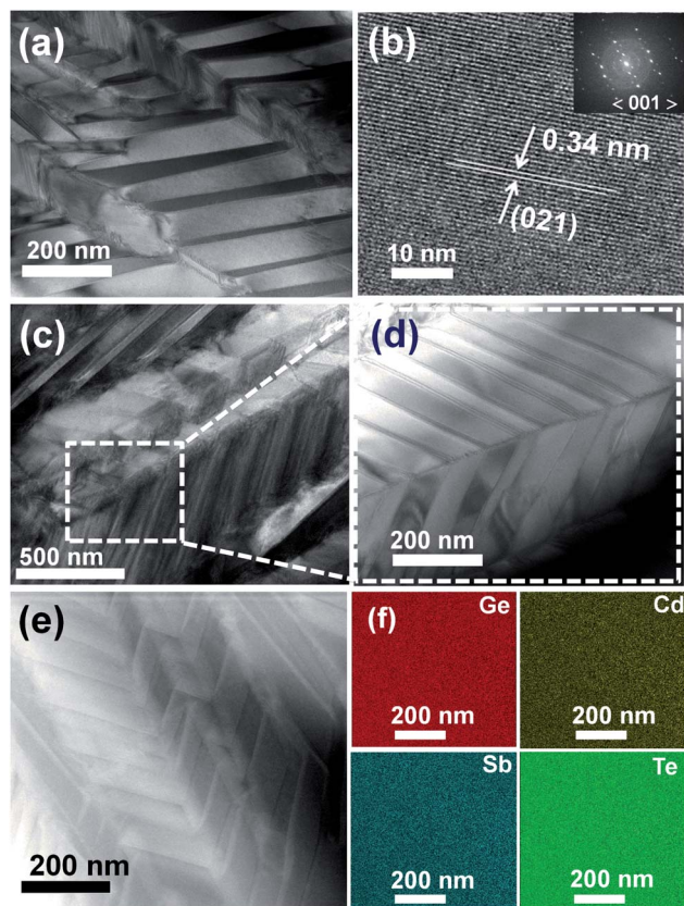
Fig. 9 (a) Low magnification TEM image of the \text{Ge}_{0.89}\text{Cd}_{0.03}\text{Sb}_{0.08}\text{Te} sample with the herringbone structure. (b) HRTEM image for (a). (c) TEM images for the \text{Ge}_{0.89}\text{Cd}_{0.03}\text{Sb}_{0.08}\text{Te} sample with different domain variants. (d) HRTEM for (c). (e) STEM image and (f) elements distribution by EDS mapping in the \text{Ge}_{0.89}\text{Cd}_{0.03}\text{Sb}_{0.08}\text{Te} sample.
