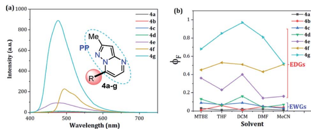
Fig. 3 (a) Emission spectra of compounds 4a–g in THF. (b) A plot of the quantum yields of probes 4a–g versus solvent ( 1 \times 10^{-5} M) at 20 °C.
