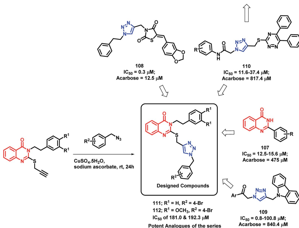
Scheme 41 Synthesis and design strategy for triazole-linked quinazolinone hybrids, targeting α-glucosidase.
