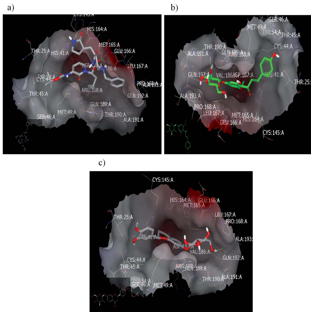
Fig. 6 Visual representation by veda for (a) \alpha -ketamide standard; (b) compound 3 ; and (c) compound 4 docked with ID:6y2f.
