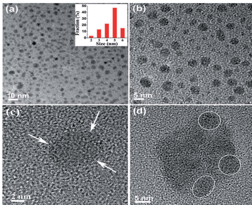
Fig. 3 (a and b) TEM images of QDs in water, inset shows size distribution of QDs in water. (c) HRTEM image of a single QD. (d) QDs in DMF show slight agglomeration. Reproduced with permission from ref. 57, copyright 2016, The Royal Society of Chemistry.
