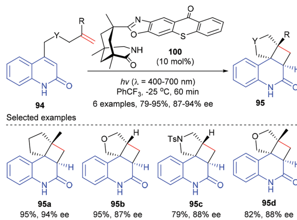
Scheme 28 Chiral thioxanthere catalyzed [2 + 2] photocycloaddition reactions of 4-tethered quinolones.
