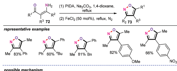
Scheme 33 Iron-catalyzed ring expansion of 2 H -azirine from enaminones.
