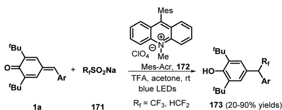
Scheme 35 Synthesis of difluoromethylated diarylmethanes.
