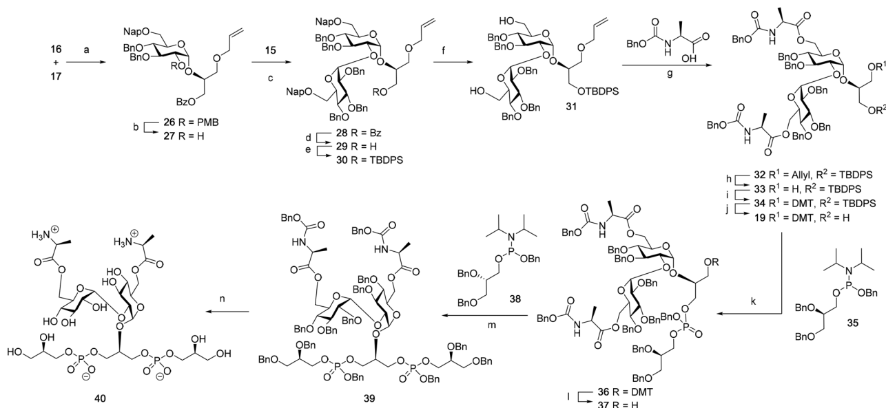
Scheme 5 Synthesis of a di-allyl- \alpha -kojibiose containing LTA fragment. (a) TMSI, \text{Ph}_3\text{P}=\text{O} , DCM, 36 h, 76%, \alpha:\beta > 20:1 . (b) TES, HCl/HFIP, DCM : HFIP = 1 : 1 (v : v), 93%. (c) DMF, TfOH, 24 h, 95%, \alpha:\beta > 10:1 . (d) \text{CH}_3\text{ONa} , DCM : \text{CH}_3\text{OH} = 1 : 1 (v : v), 92%. (e) TBDPSCl, imidazole, DMF, 99%. (f) DDQ, DCM : \text{H}_2\text{O} = 10 : 1 (v : v), 77%. (g) PyBOP, NMI, DCM, 90%. (h) (1) \text{Ir}(\text{COD})(\text{Ph}_2\text{MeP})_2\text{PF}_6 ; (2) \text{I}_2 , \text{NaHCO}_3 , \text{H}_2 , THF, 85%. (i) \text{DMTrCl} , DIPEA, DCM, 95%. (j) HF-pyridine, THF/pyridine, 86%. (k) 1) DCl, \text{CH}_3\text{CN} ; (2) CSO. (l) TsOH, DCM/ \text{CH}_3\text{OH} = 1 : 1 (v : v), 93%. (m) DCl, \text{CH}_3\text{CN} ; (2) CSO, 88%. (n) \text{H}_2 , Pd/C, dioxane/ \text{H}_2\text{O} = 2 : 1 (v : v), 3 day, 95%.
