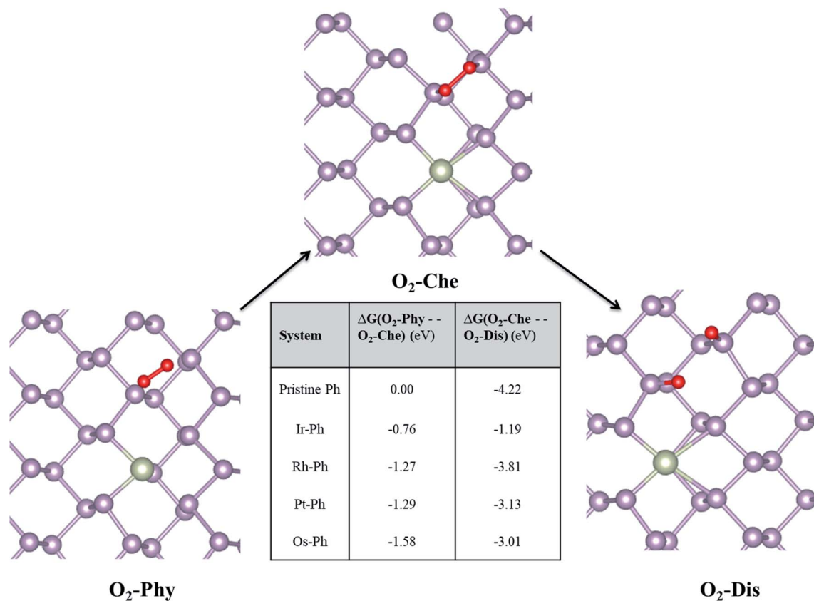
Fig. 8 Free energy analysis of \text{O}_2 interaction with TM-Ph SACs. Pristine phosphorene is the reference system. \text{O}_2 -Phy, \text{O}_2 -Che, and \text{O}_2 -Dis represent the physisorbed, chemisorbed and dissociated oxygen molecule, respectively.
