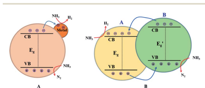
Fig. 2 Illustrations of metal-loading (A) and heterojunction building (B) for enhanced photocatalytic ammonia decomposition performance.
