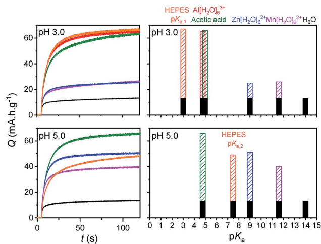
Fig. 7 (Left) Charge stored over the time course of reductive potential step chronoabsorptometry experiments performed at GLAD-TiO 2 /TiO 2 /ITO electrodes in different aqueous electrolytes adjusted to pH 3.0 or 5.0 (the pH values are reported on the graphs): (black) 0.3 M KCl, (blue) 0.25 M ZnCl 2 , (magenta) 0.25 M MnCl 2 , (red) 0.25 M AlCl 3 , (green) 0.3 M KCl + 0.25 M acetic acid, and (orange) 0.3 M KCl + 0.25 M HEPES. The applied potential during the experiments was -0.82 V at pH 3.0 and -0.94 V at pH 5.0 (vs. Ag/AgCl). (Right) Maximal charge stored as a function of pH and pK a of the proton donor. The black dense bar areas correspond to the charge stored at the electrical double layer (recovered from the experiment conducted in a 0.3 M KCl aqueous electrolyte), while the dashed areas correspond to the equilibrium charge stored through the faradaic reduction of TiO 2 coupled to proton-ion insertion.
