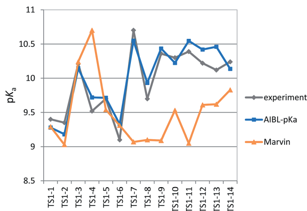
Fig. 5 Relative pK_a values of the primary sulfonamide group across the series TS1-1 to TS1-14 . Although Marvin's performance in terms of mean absolute error evaluation is good (0.65), AIBL- pK_a manages to closely match the overall trend in the magnitude of pK_a values across the series.
