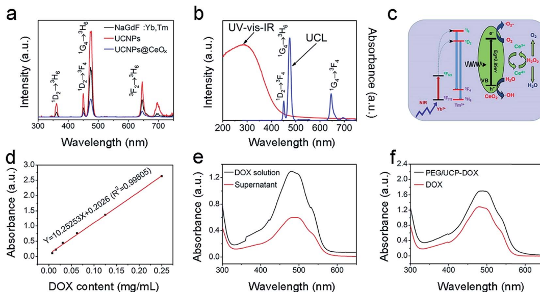
Fig. 3 Upconversion emission spectra of the \text{NaGdF}_4\text{:Yb,Tm} core NPs, UCNPs, and UCNPs@mCeO x (a). The UV-vis-IR DRS and UCL of the UCNPs@mCeO x (b). Schematic illustration of the UC, photocatalysis, and enzyme-like catalysis mechanism of the UCNPs@mCeO x (from left to right) (c). The standard curve for DOX solution detected at 480 nm (d). The absorption spectra of the initial DOX solution and supernatant obtained after coating the drug (e). UV-vis absorption spectra of the DOX molecules and the final PEG/UCP-DOX (f).
