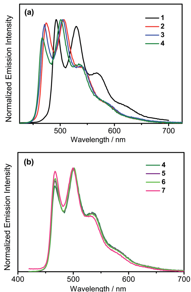
Fig. 3 (a) Normalized emission spectra of (a) 1–4 and (b) 4–7 in dichloromethane solution at 298 K.
