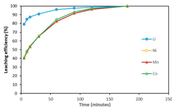
Fig. 3 Leaching kinetics of NMC 811 in 4 \text{ mol } L^{-1} HCl at S/L = 20 \text{ g } L^{-1} and 25^\circ\text{C} .
